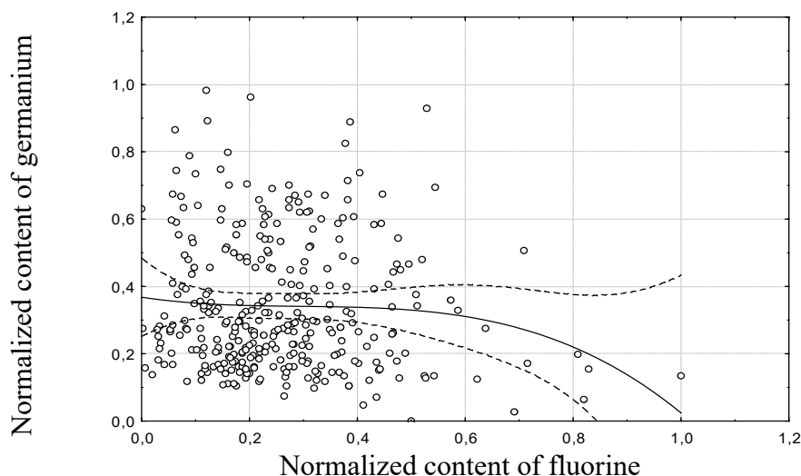
Figure 4 – The result of the regression analysis of modeling the polynomial relationship between the normalized germanium content and the normalized fluorine content
