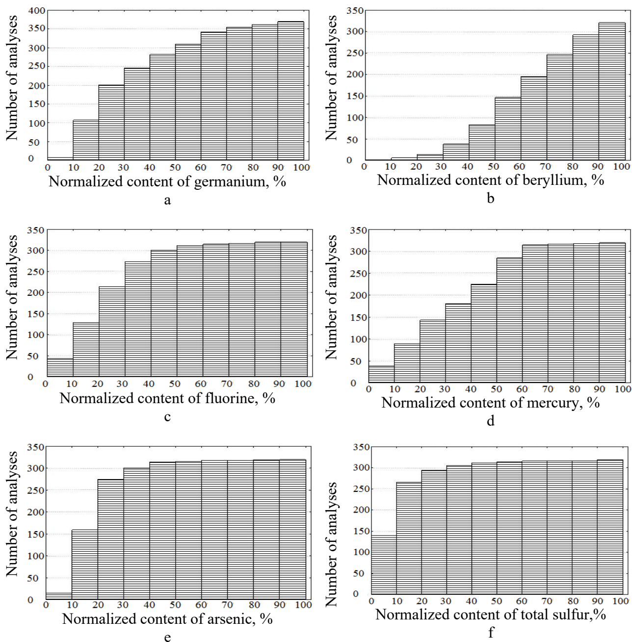
Figure 1 – Cumulative histograms of normalized content values
